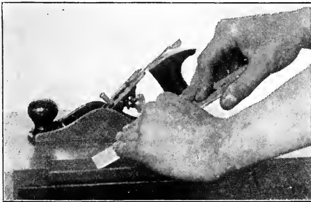
Fig. 107—Whetting Plane Bit
